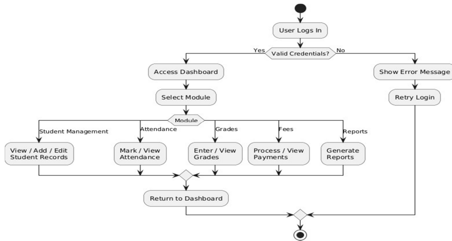
Fig1. Pupil Management Software Flowchart
