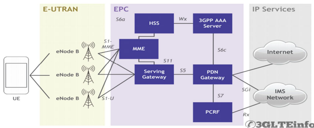
Fig 1. 4G/LTE Architecture
