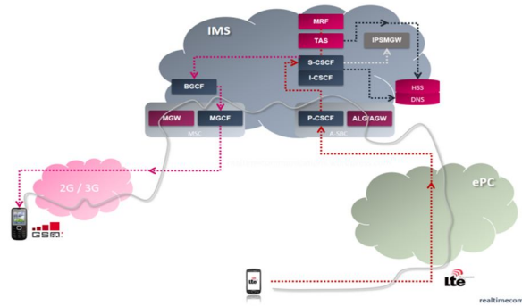
Fig 2. VoLTE Architecture
