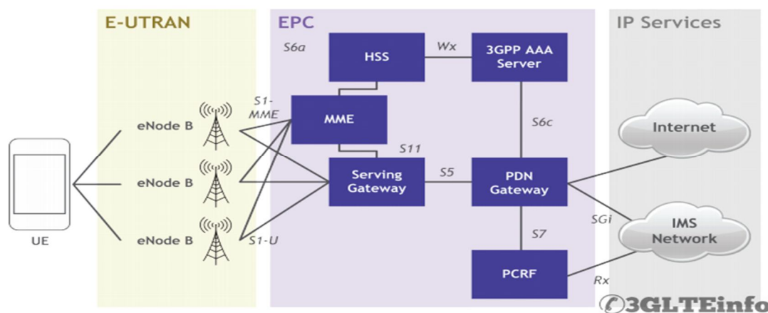
Fig 1. 4G/LTE Architecture
