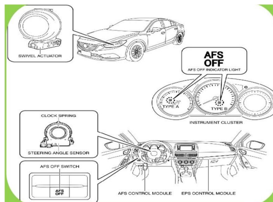
Fig 3: AFS and EFS control module
