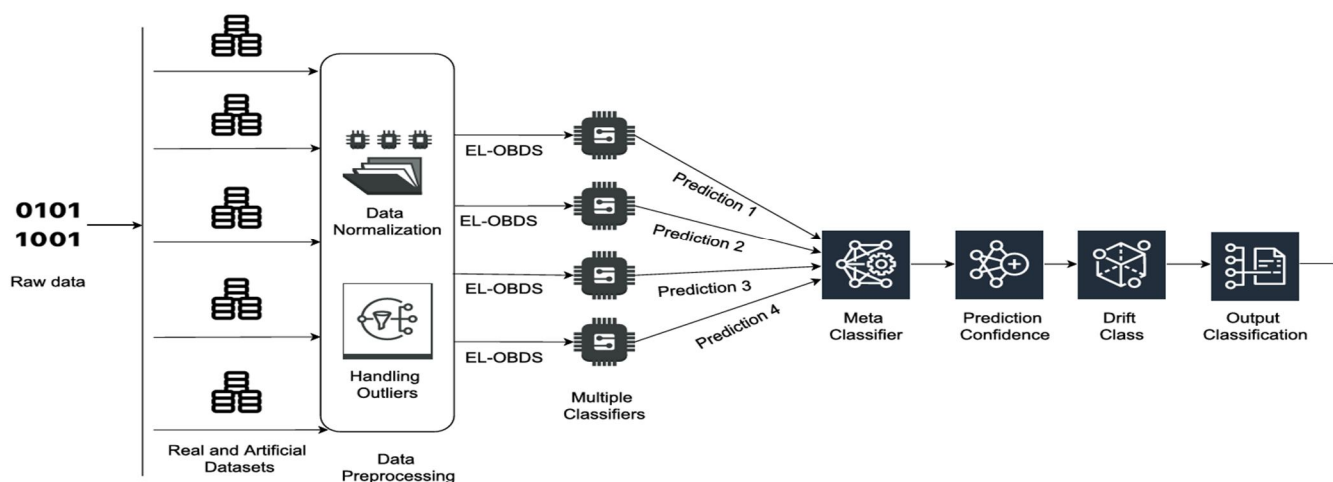
Figure 2: Dynamic ensemble weighting mechanism for concept drift adaptation [6]
