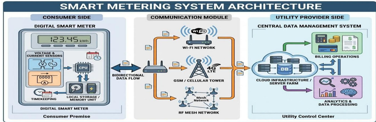
Figure 1: Smart Metering System Architecture showing the integration of digital meters, communication modules, and data management systems.
