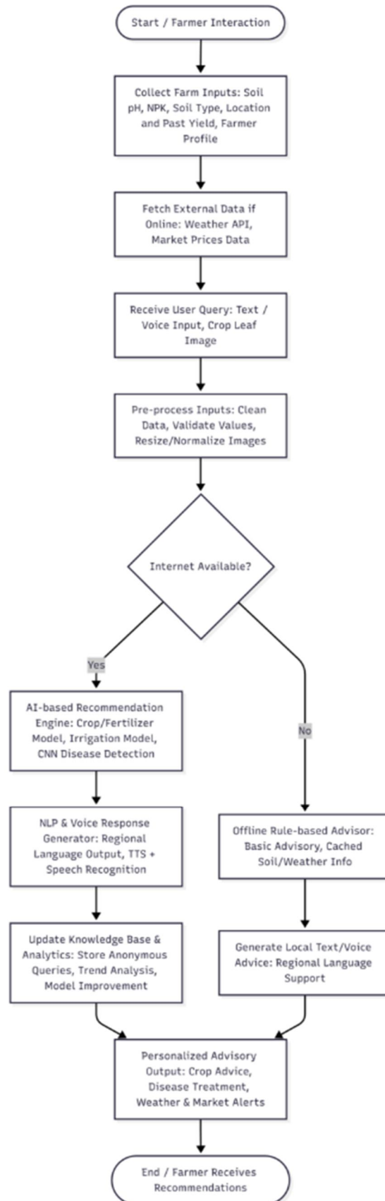
Fig. 1: AgroAI system architecture and data flow
