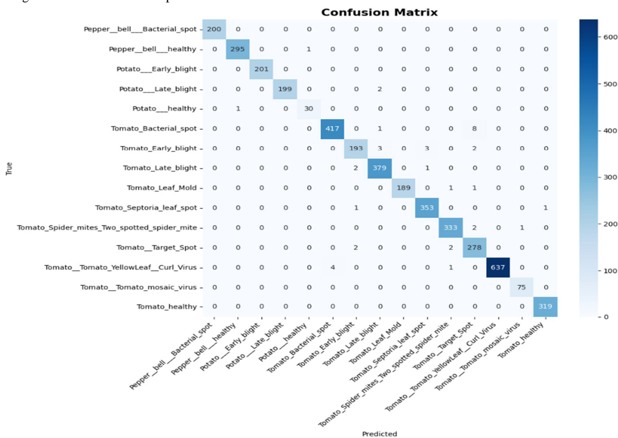
Fig. 2: Confusion Matrix of Test Results.
