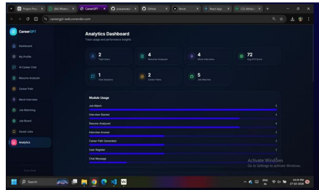
Fig. 7. Analytics Dashboard
