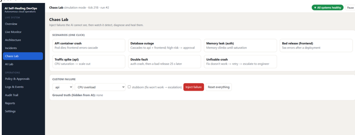
Fig. 6. Chaos Lab page: one-click fault scenarios and custom failure injection.
