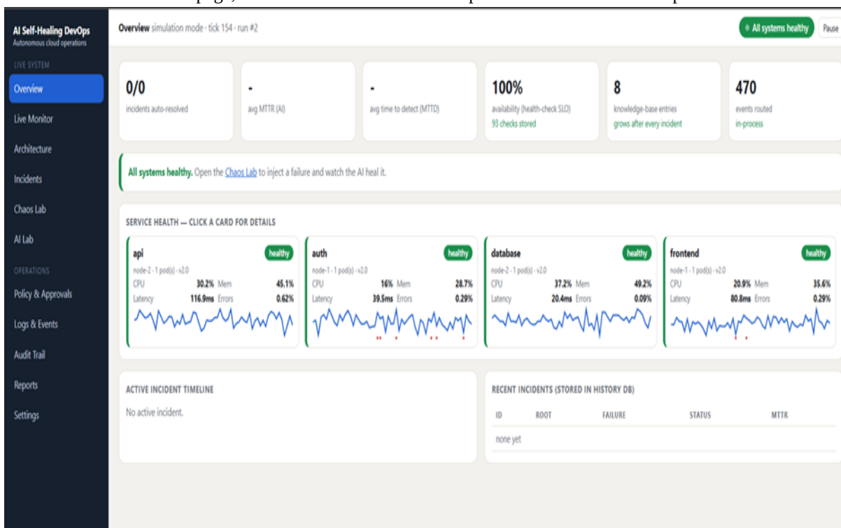
Fig. 4. Overview page: incident statistics, service health cards, active incident timeline and recent incidents.
