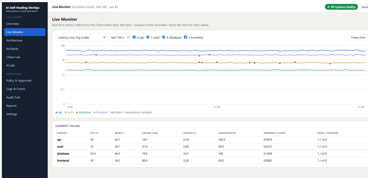
Fig. 5. Live Monitor page: real-time service metrics with Isolation Forest anomalies marked as red dots.
