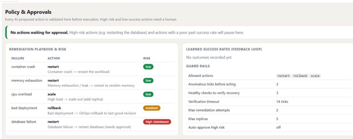
Fig. 3. Policy & Approvals page: remediation playbook and risk levels, learned success rates and guard rails.
