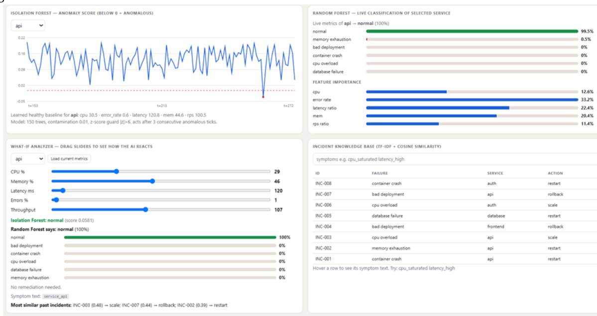
Fig. 2. AI Lab page: Isolation Forest anomaly score, Random Forest classification with feature importance, what-if analyzer and incident knowledge base retrieval.
