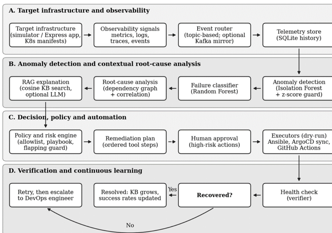
Fig. 1. Block diagram of the AI Self-Healing DevOps framework.
