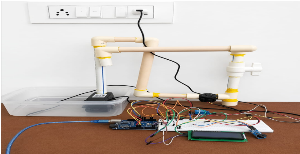
Fig.2 AI – Based Hydraulic Leak Detection System
