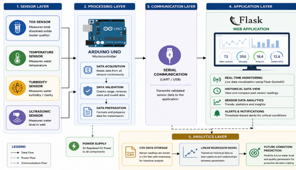
Figure 1. System Architecture of AI-Powered Water Well Analysis with IoT and Machine Learning
