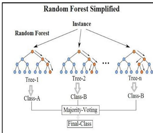
Fig. 7. Random Forest Simplified [16].
