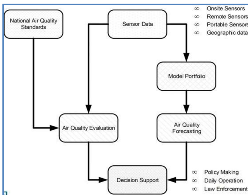
Fig. 1. Big data based decision support for air quality [7].
