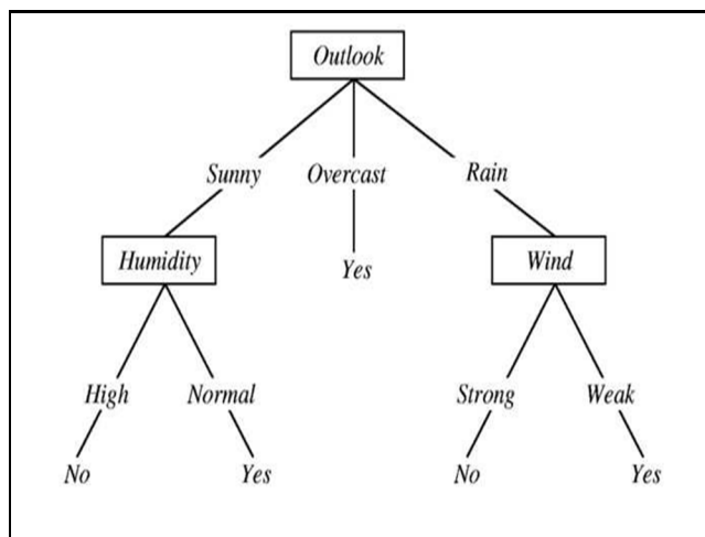
Fig. 8. Decision tree algorithm [18].
