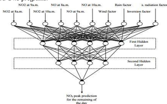
Fig. 5. ANN model for air quality [14].
