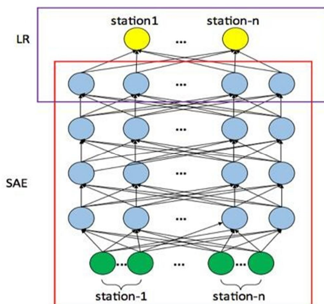
Fig10 AP-LSSVM air modelling quality prediction
