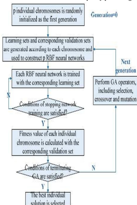
Fig. 6. Flow of genetic algorithm based ANN [15].
