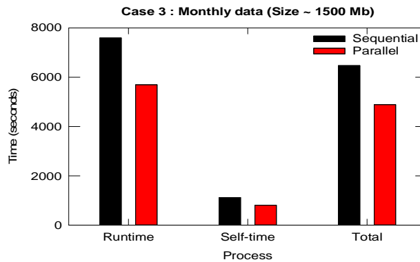
Fig.6.1 Time Taken to Process Monthly Data in Sequential (Black Colour) and Parallel (Red)
