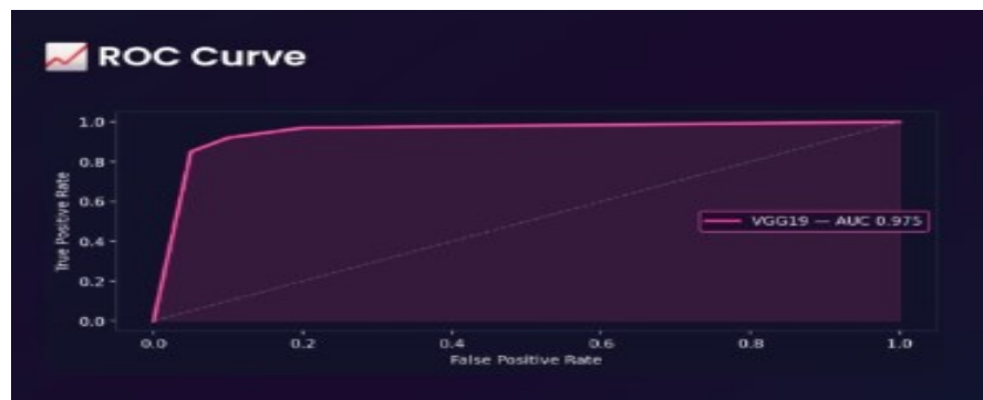
Fig.6.ROC Curve
