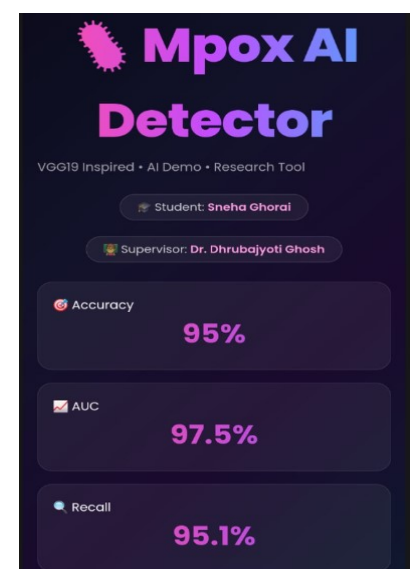
Fig.1. System Overview
