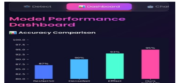
Fig.4.ModelPerformance Dashboard
