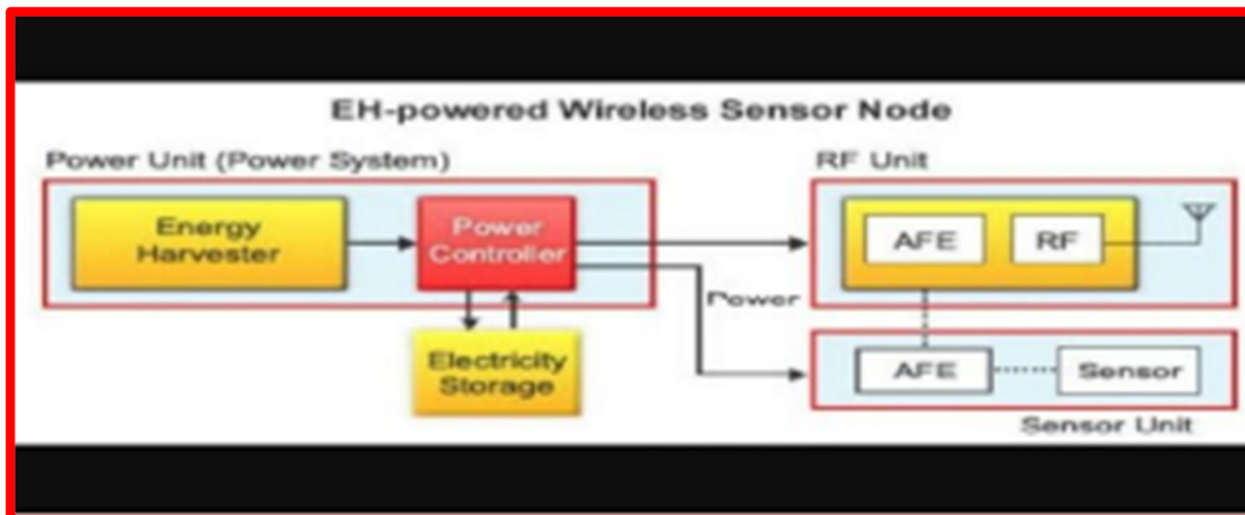
Fig.14: Wireless Sensors
