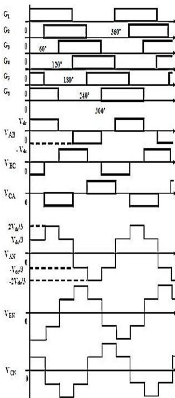
Fig: 4 Conduction of inverter
