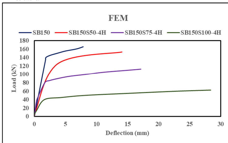
Fig. 19: Comparison of Numerical Load-Deflection Curves of Steel Beams
