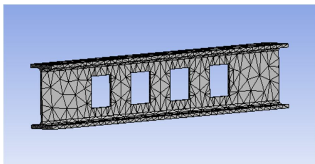
Fig. 13: FE Discretization of SB150S75-4H
