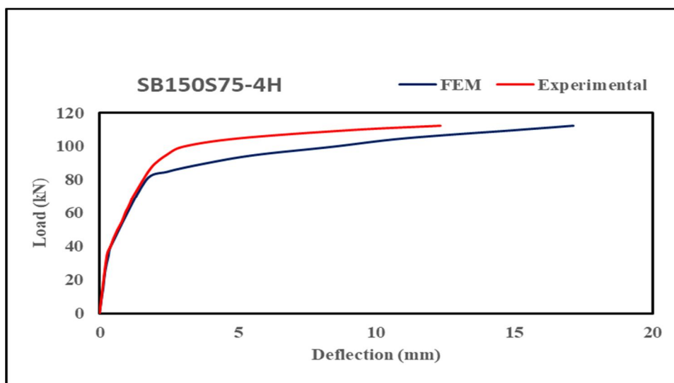
Fig. 22: Experimental and Numerical Load-Deflection Curves of SB150S75-4H
