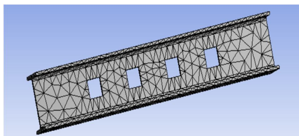
Fig. 12: FE Discretization of SB150S50-4H
