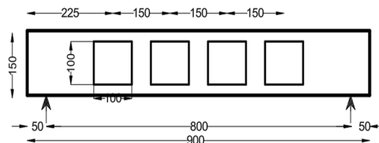
Fig. 6: Dimensions of SB150S100-4H
