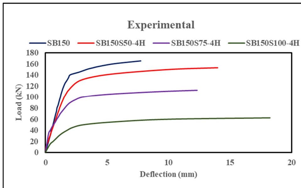
Fig. 18: Comparison of Experimental Load-Deflection Curves of Steel Beams
