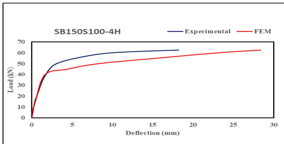
Fig. 23: Experimental and Numerical Load-Deflection Curves of SB150S100-4H
