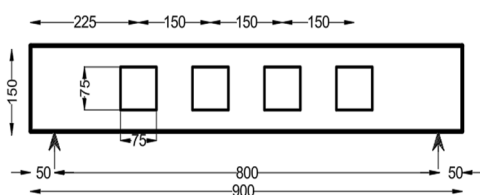
Fig. 5: Dimensions of SB150S75-4H
