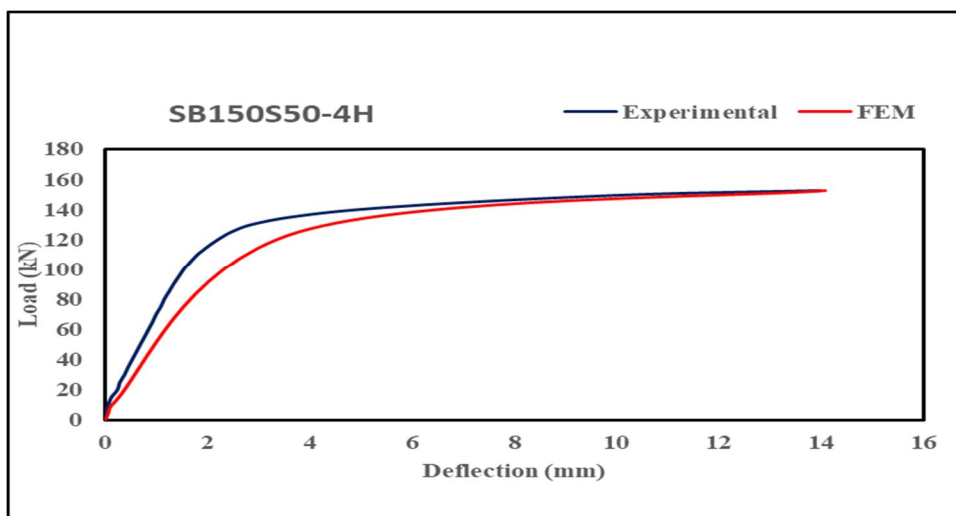
Fig. 21: Experimental and Numerical Load-Deflection Curves of SB150S50-4H
