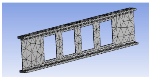
Fig. 14: FE Discretization of SB150S100-4H
