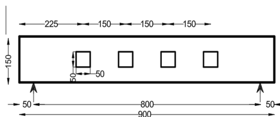
Fig. 4: Dimensions of SB150S50-4H
