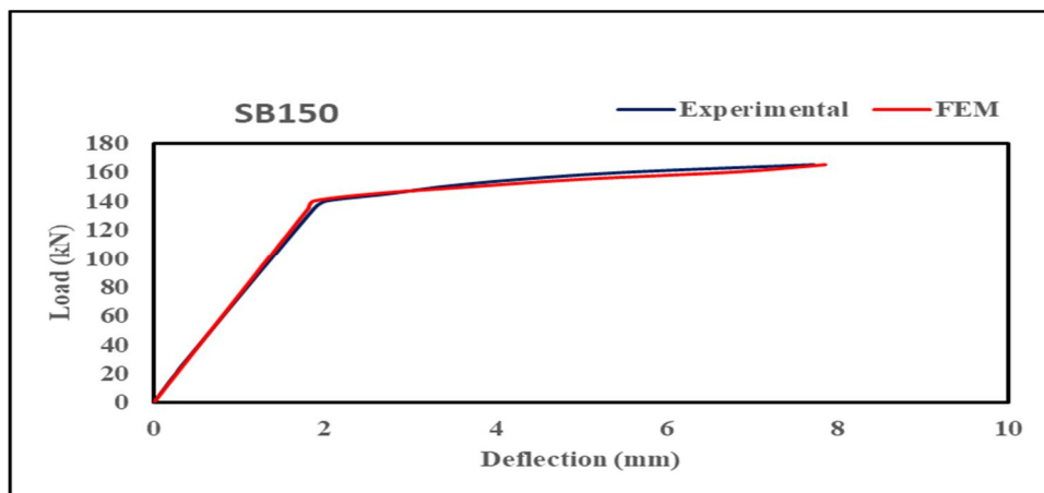
Fig. 20: Experimental and Numerical Load-Deflection Curves of SB150
