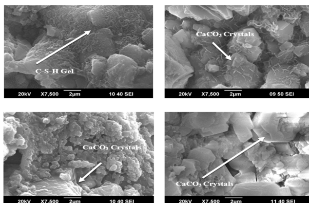
Figure 7: 7 days bacterial concrete effects on SEM
