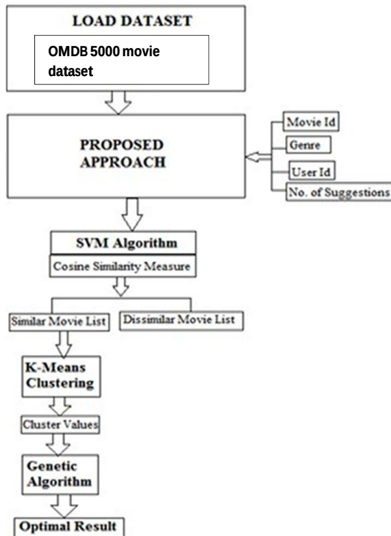
Fig 2. Proposed Approach
