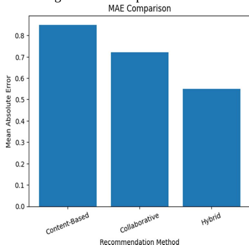
Fig. 5 MAE Comparisons
