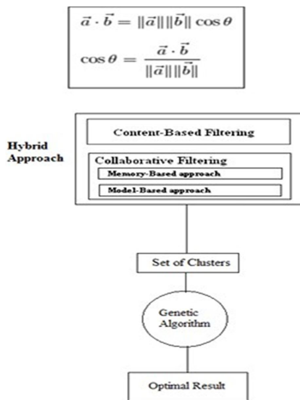
Fig 1. Hybrid Approach with Genetic Algorithm
