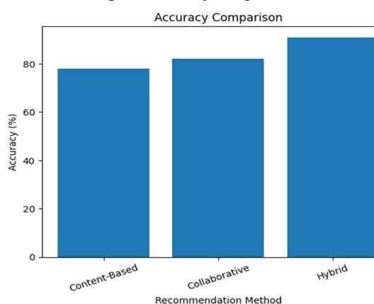
Fig. 3 Accuracy Graph
