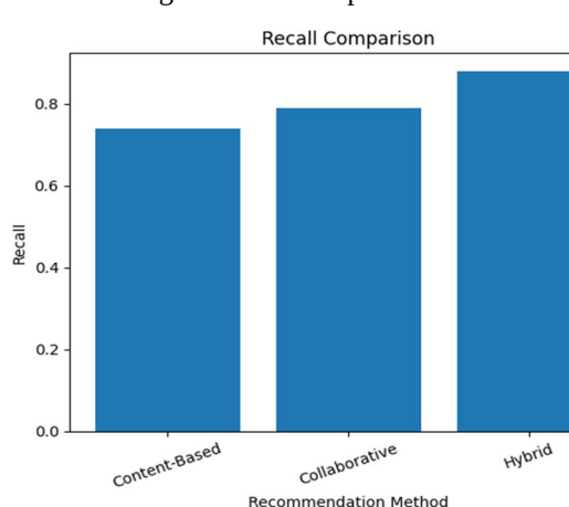
Fig. 6 Recall Comparisons
