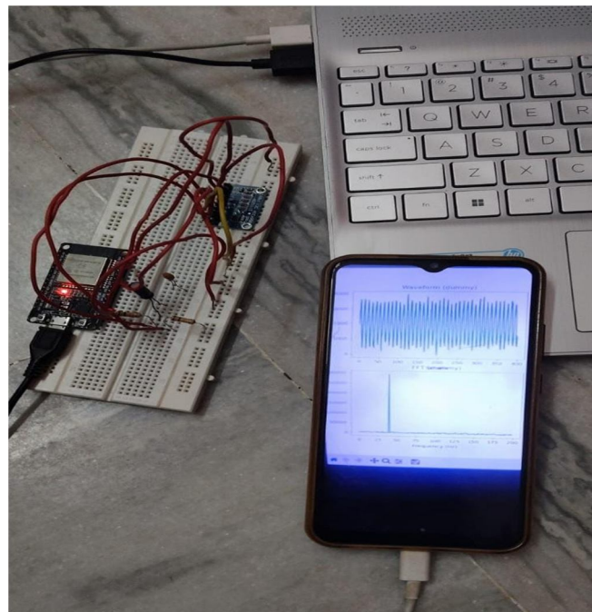
Fig. 3 Hardware Implementation
