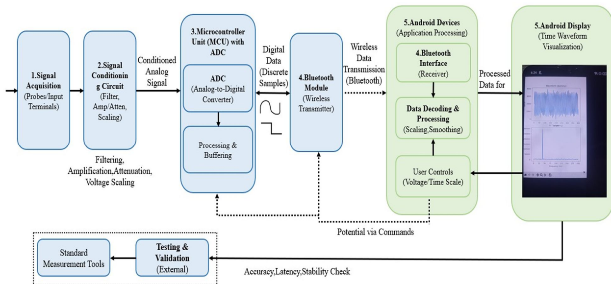
Fig. 1 Block Diagram of Portable Android Oscilloscope
