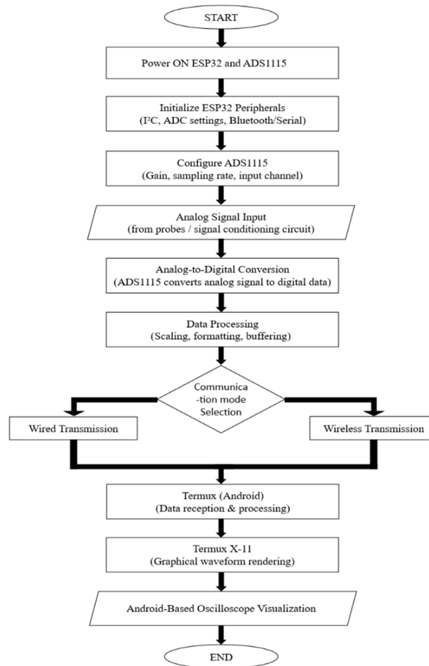
Fig. 2 Flow Diagram of Portable Android Oscilloscope
