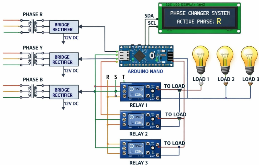
Fig. – Circuit Diagram of Arduino-Base Automatic Phase Shifter
