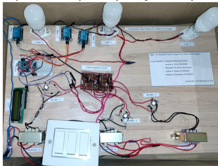
Fig. Hardware Setup of Arduino-Based Automatic Phase Shifter
