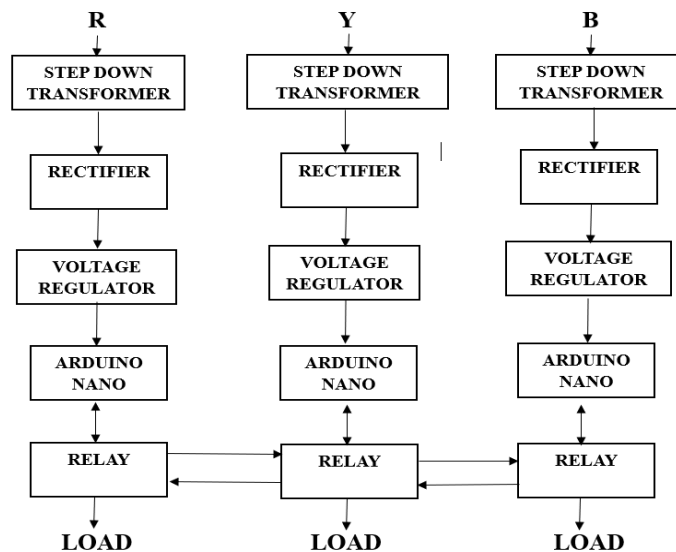
Fig. Block Diagram of Arduino-Based Automatic Phase Shifter
