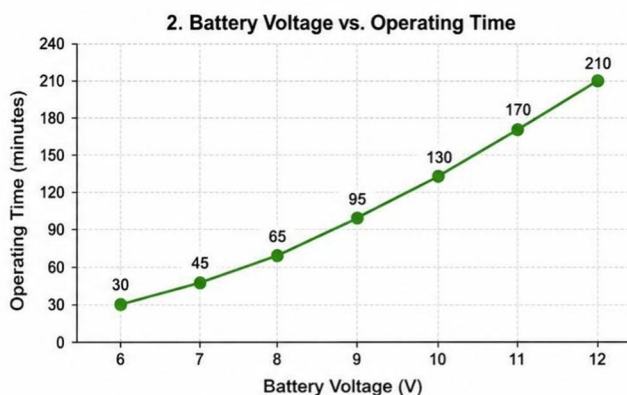
FIG. 3: Battery Voltage vs Operating Time
