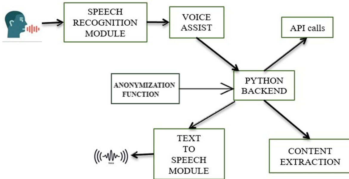
Fig 2 : Workflow model
