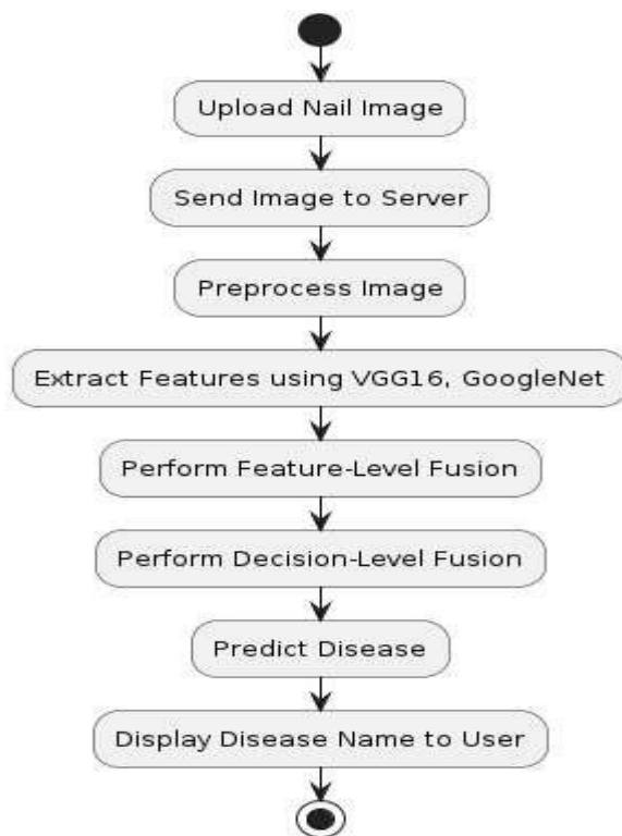
Fig 2: Activity diagram
