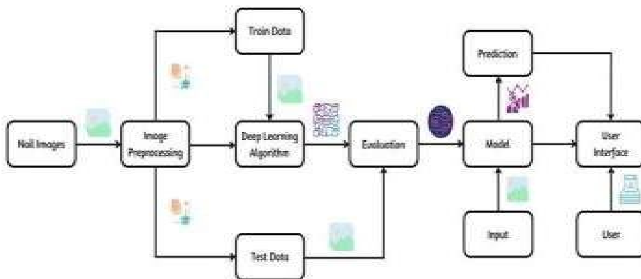
Fig 1: System Architecture
