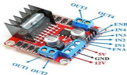
Fig.4 L298N Motor Driver
