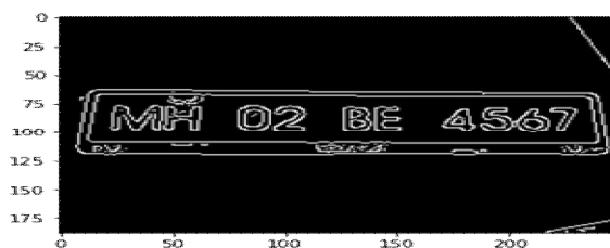
Figure 5 – Canny Edge Detection on Masked Image
