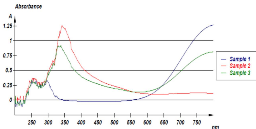
Figure-2: UV-Vis Spectrophotometer Analysis of (sample-3) Punica granatum peel Extract, (sample-1) ZnSO 4 , (sample-2) ZnNps.
