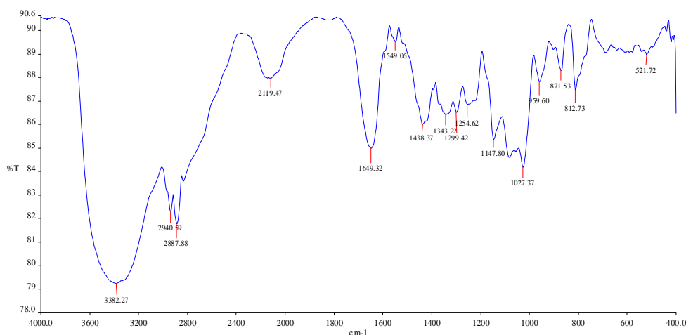
Figure-3: FTIR Analysis of ZnO nanoparticles of Punica granatum peels extract.
