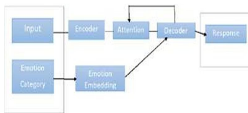
Fig5. Architecture Diagram
