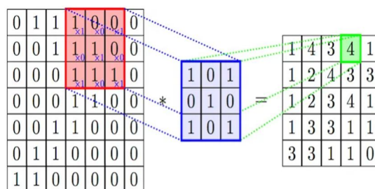
Fig 1. Convolution Operation
