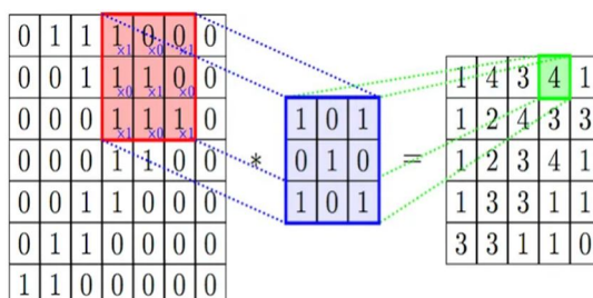
Fig 1. Convolution Operation
