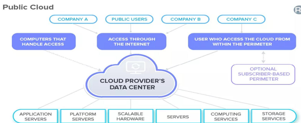
FIG II: PUBLIC CLOUD
