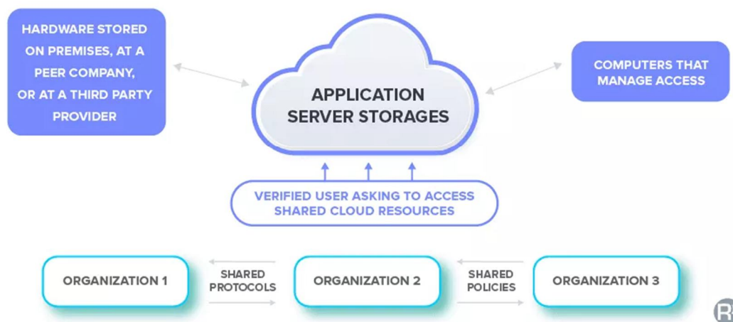
FIG V: COMMUNITY CLOUD
