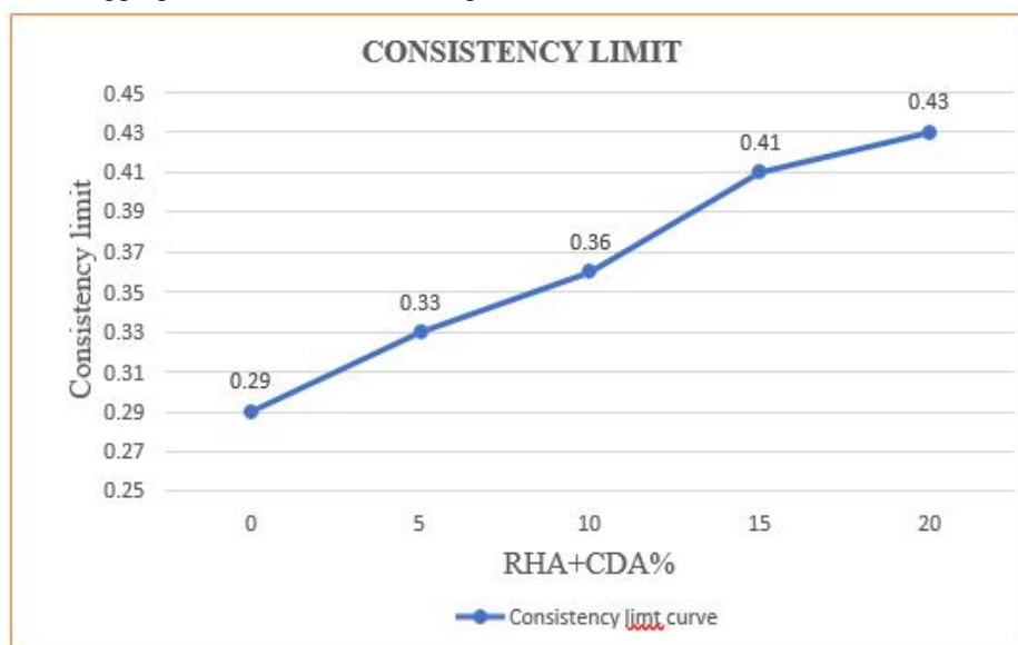
Fig. 3: Consistency curve for RHA+CDA concrete mix
