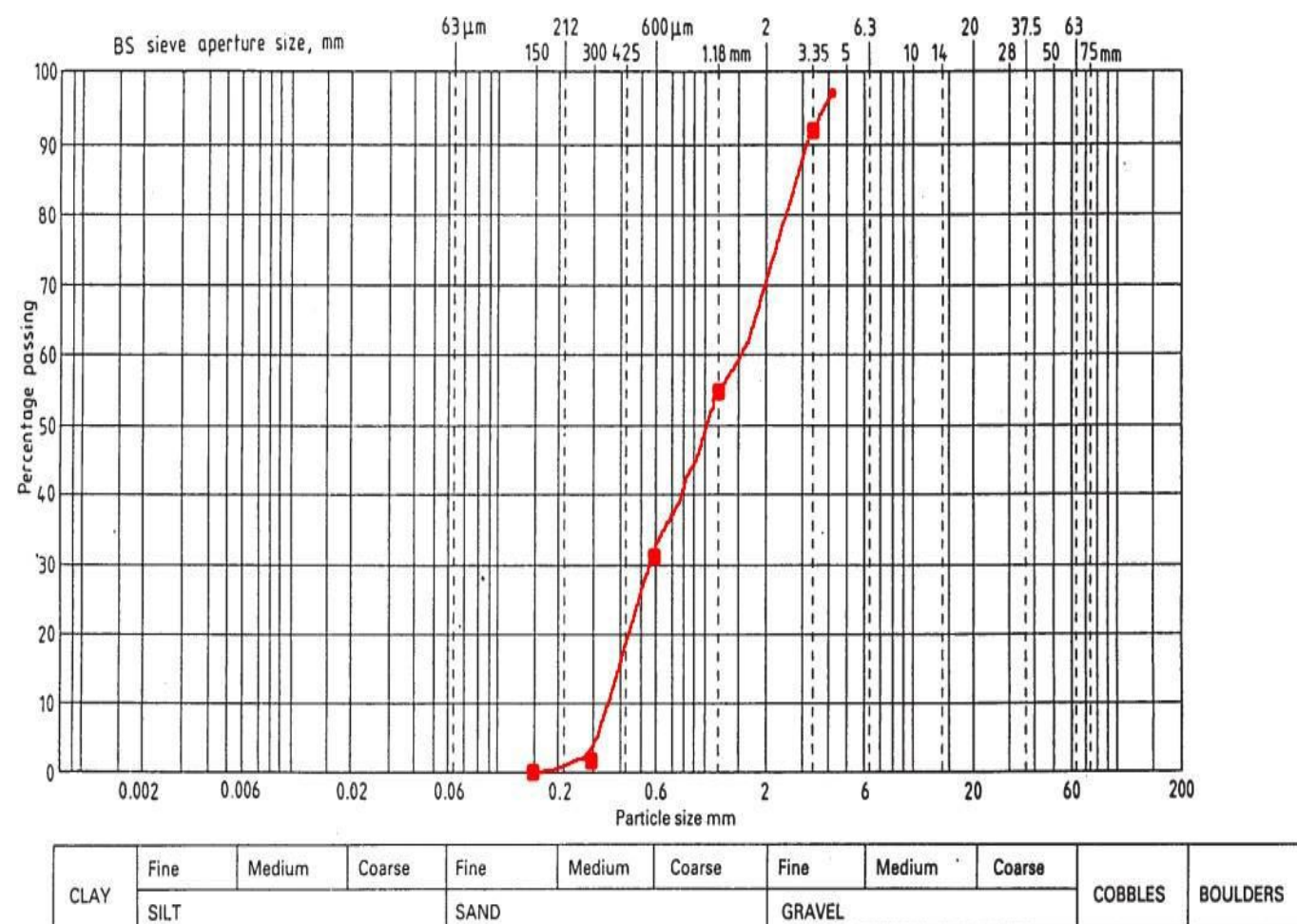
Fig. 4: Gradation Curve for Fine Aggregate
