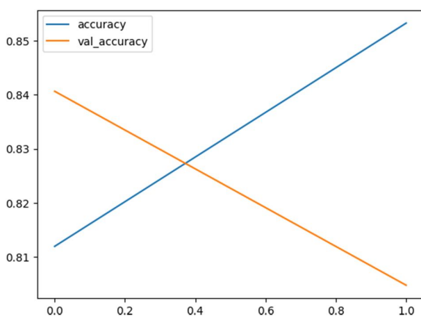
Validation Accuracy
