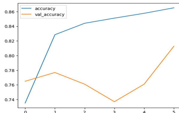
Validation Accuracy
