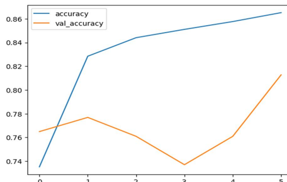
Validation Accuracy
