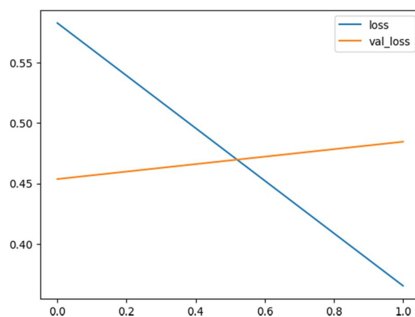
Validation Loss
