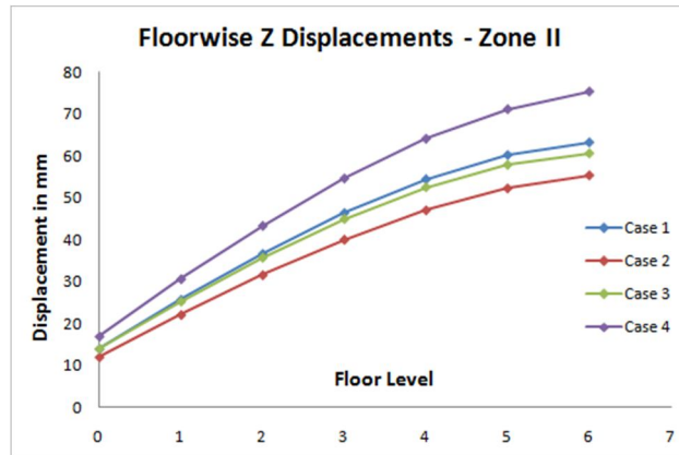
Figure-11 Z displacement for Zone II (Corner column)
