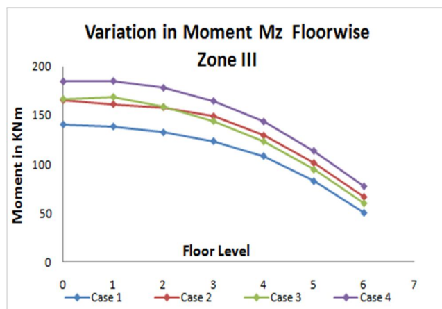
Figure-28 Moment Mz for Zone III (Corner Column)
