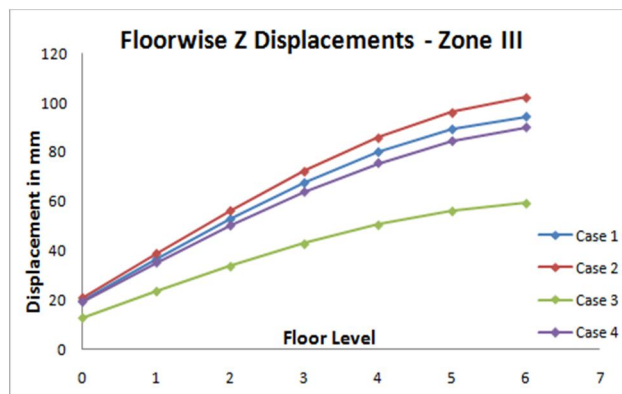
Figure-12 Z displacement for Zone III (Corner column)
