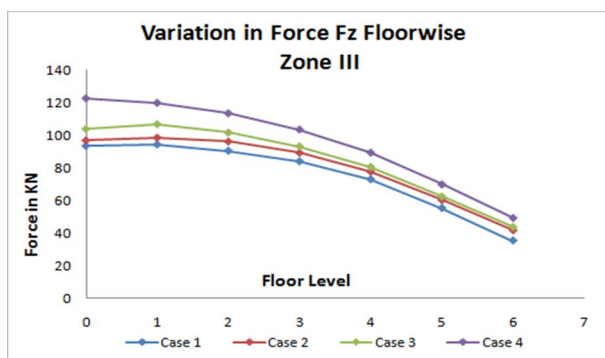
Figure-22 Shear Force Fz for Zone III (Intermediate Column)
