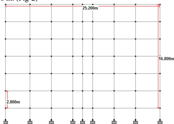
Figure-2 Elevation of Structure
