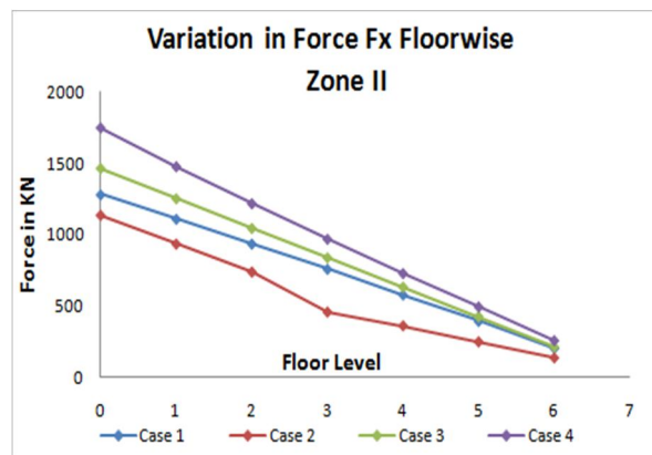
Figure-15 Axial Force Fx for Zone II (Corner Column)
