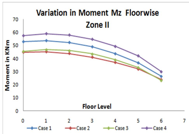
Figure-33 Moment Mz for Zone II (Intermediate Beam)
