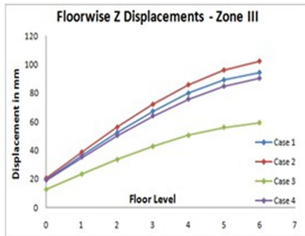
Figure-14 Z displacement for Zone III (Intermediate Column)
