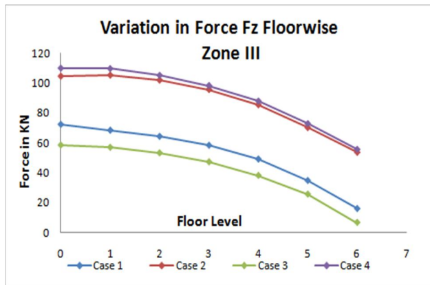
Figure-20 Shear Force Fz for Zone III (Corner Column)
