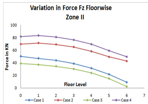
Figure-19 Shear Force Fz for Zone II (Corner Column)
