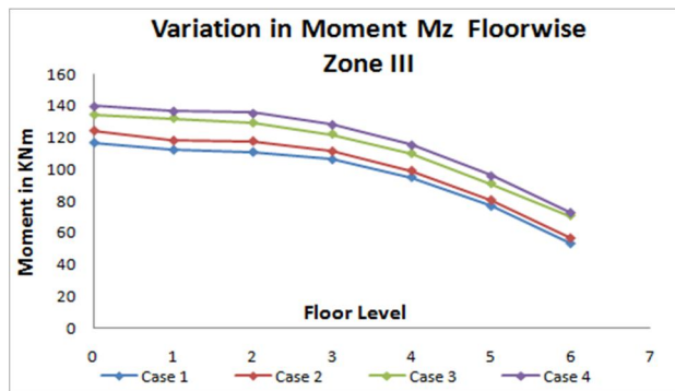
Figure-30 Moment Mz for Zone III (Intermediate Column)
