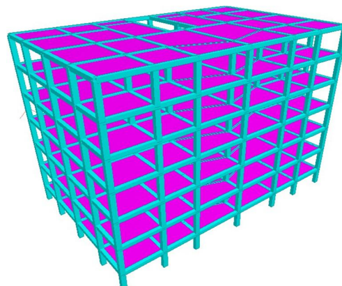
Figure-3 3D view of Structure (case 1)
