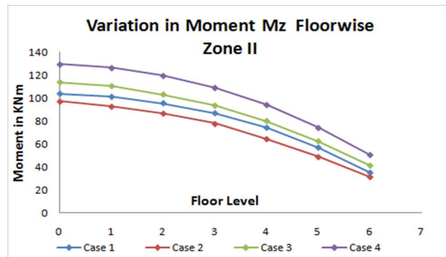
Figure-27 Moment Mz for Zone II (Corner Column)
