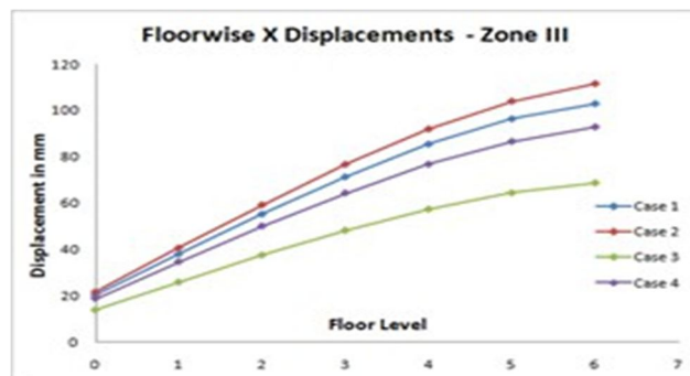
Figure-10 X displacement for Zone III (Intermediate Column)
