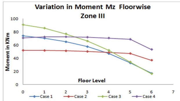
Figure-32 Moment Mz for Zone III (Corner Beam)
