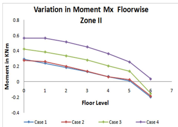
Figure-23 Moment Mx for Zone II (Corner Column)
