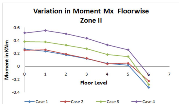
Figure-25 Moment Mx for Zone II (Intermediate Column)
