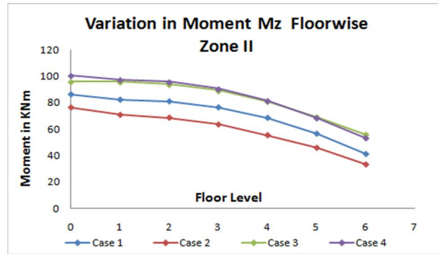
Figure-29 Moment Mz for Zone II (Intermediate Column)
