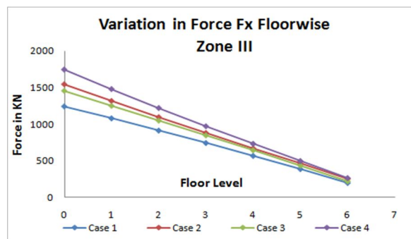
Figure-16 Axial Force Fx for Zone III (Corner Column)
