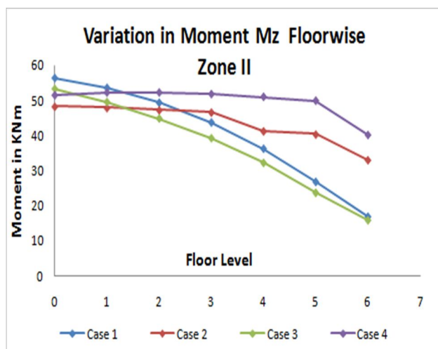
Figure-31 Moment Mz for Zone II (Corner Beam)
