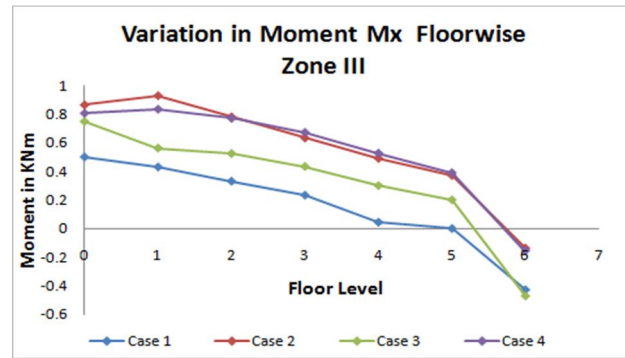
Figure-26 Moment Mx for Zone III (Intermediate Column)
