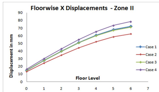
Figure-7 X displacement for Zone II (Corner Column)
