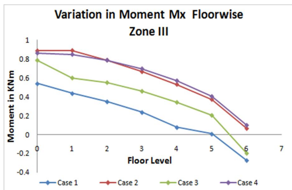
Figure-24 Moment Mx for Zone III (Corner Column)
