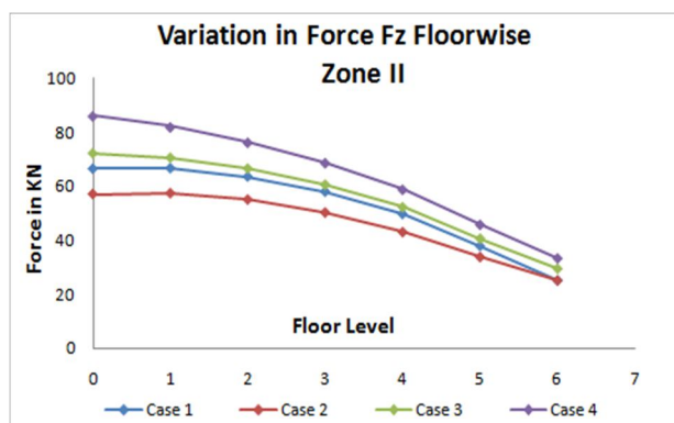
Figure-21 Shear Force Fz for Zone II (Intermediate Column)
