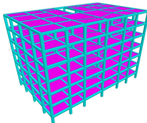
Figure-3 3D view of Structure (case 1)
