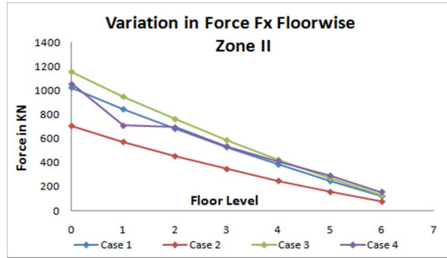
Figure-17 Axial Force Fx for Zone II (Intermediate Column)
