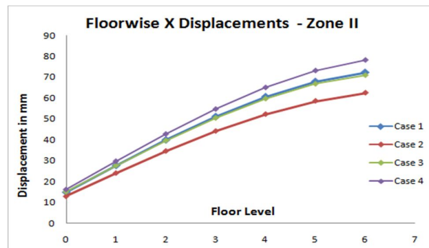
Figure-9 X displacement for Zone II (Intermediate Column)
