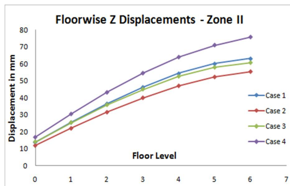
Figure-13 Z displacement for Zone II (Intermediate Column)
