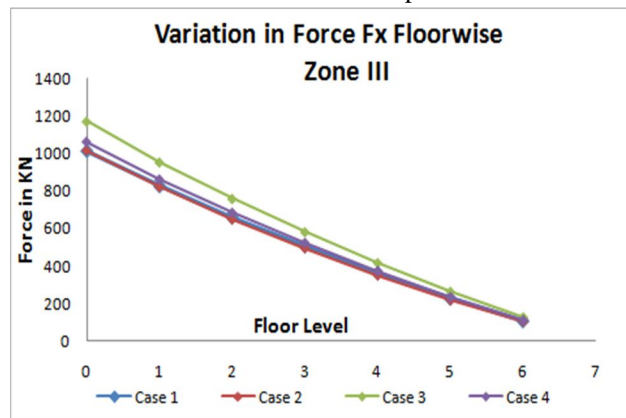
Figure-18 Axial Force Fx for Zone III (Intermediate Column)
