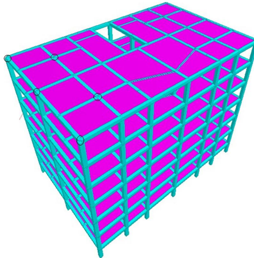
Fig-6 External and Internal Floating Column (case 4)
