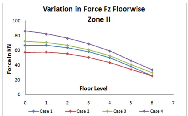
Figure-21 Shear Force Fz for Zone II (Intermediate Column)
