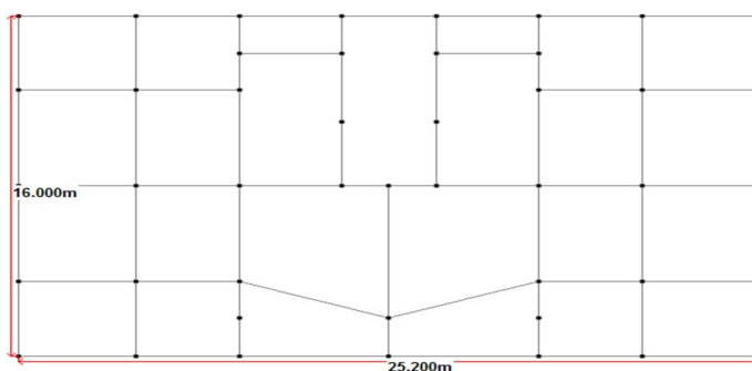
Figure-1 Plan of Structure
