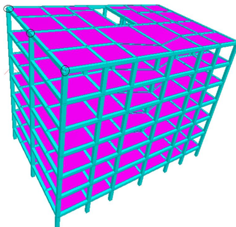
Figure-4 External Floating Column (case 2)
