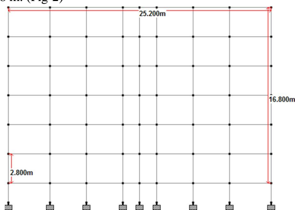
Figure-2 Elevation of Structure
