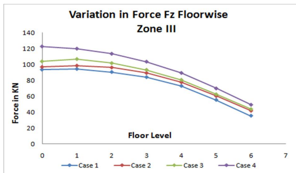
Figure-22 Shear Force Fz for Zone III (Intermediate Column)
