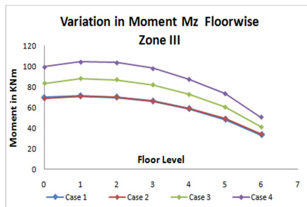
Figure-34 Moment Mz for Zone III (Intermediate Beam)
