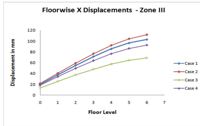
Figure-8 X displacement for Zone III (Corner Column)
