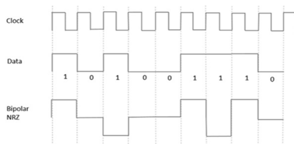
Fig 4: Bipolar NRZ coding
