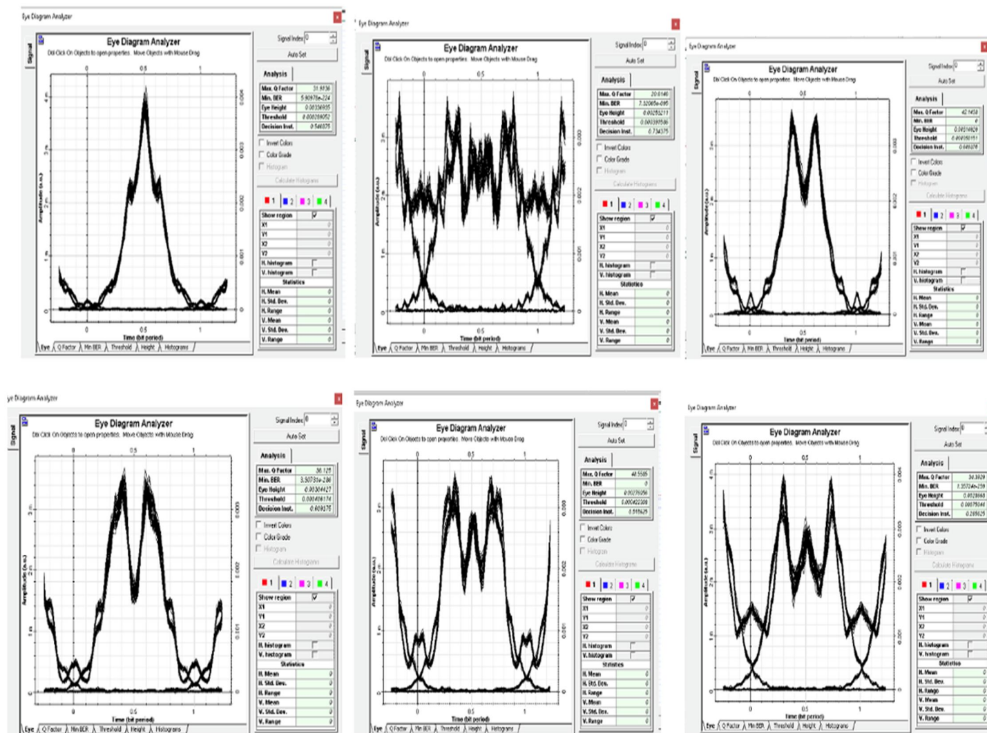
Fig 12: Eye Diagram Results
