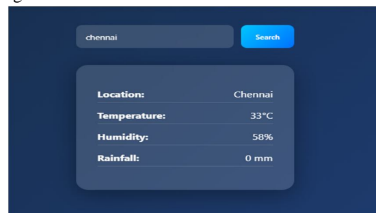
Fig. 6 Weather Prediction
