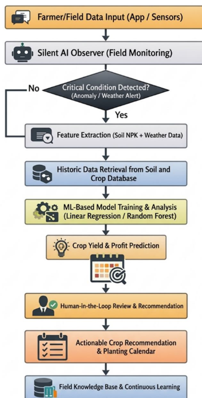
Fig. 1 Methodological Workflow
