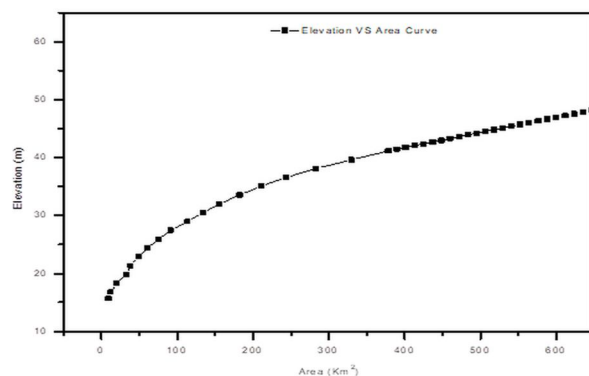
Fig. 3 Elevation–area curve of the Polavaram reservoir used as input for the storage area in HEC-RAS (data from the Water Resources Department, Polavaram Irrigation Project Headwork Circle).
