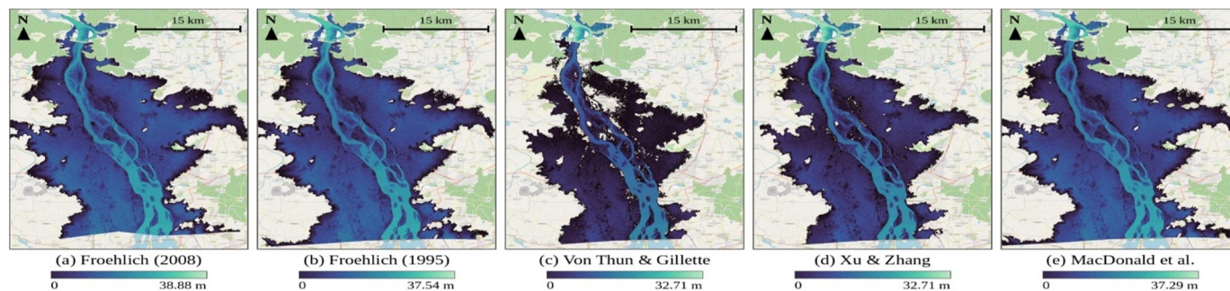
Fig. 8 Maximum flood depth maps for overtopping failure: (a) Froehlich (2008), (b) Froehlich (1995), (c) Von Thun & Gillette, (d) Xu & Zhang, and (e) MacDonald et al. The colour scale runs from 0 to the maximum depth given below each panel.
