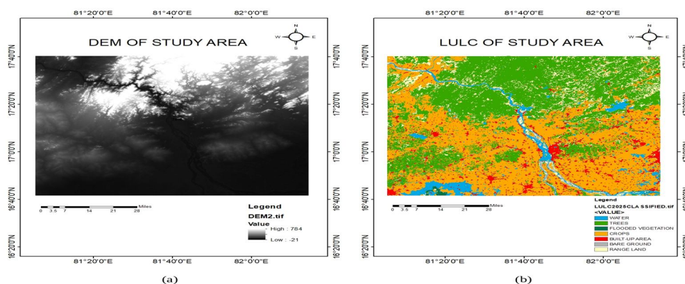
Fig. 2 Data used in the study: (a) SRTM 30 m digital elevation model (elevation in m) and (b) Esri land use and land cover of the study area.
