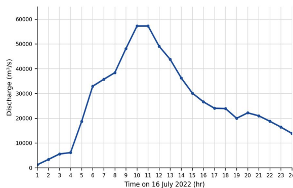
Fig. 4 Lateral inflow hydrograph of the Polavaram Dam for 16 July 2022 (data from the Water Resources Department, Polavaram Irrigation Project Headwork Circle).
