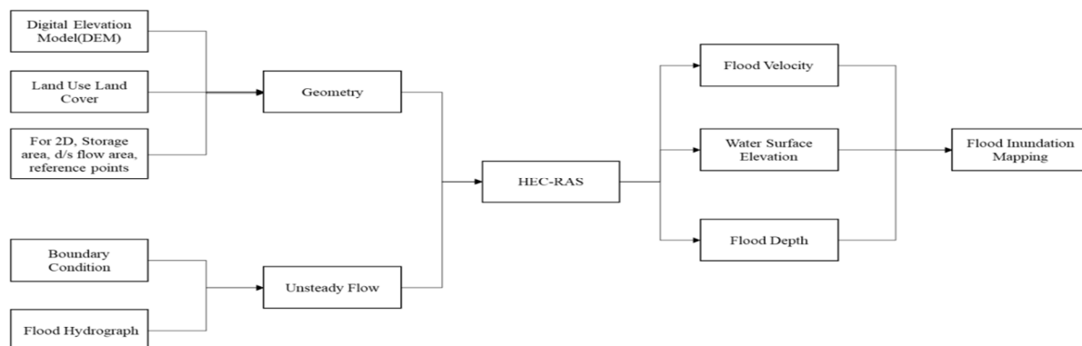
Fig.5 Methodology flow chart of the dam break analysis and flood inundation mapping.
