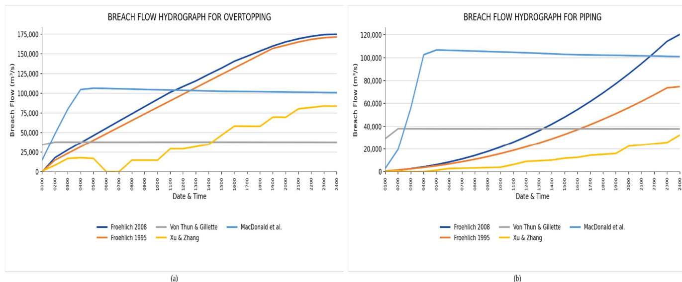
Fig. 7 Breach flow hydrographs of the five breach methods for (a) overtopping and (b) piping failure of the Polavaram Dam.
