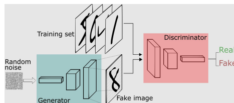
Fig. 2 Basic Structure of GANs Model[6]
