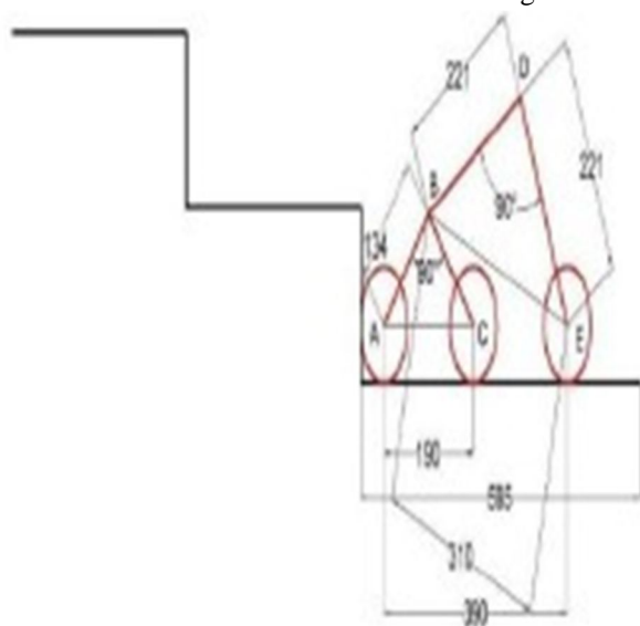
Fig.2. Cad drawing for first triangle
