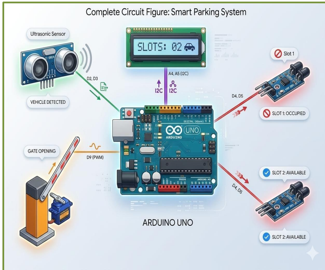
Fig. 1 System design
