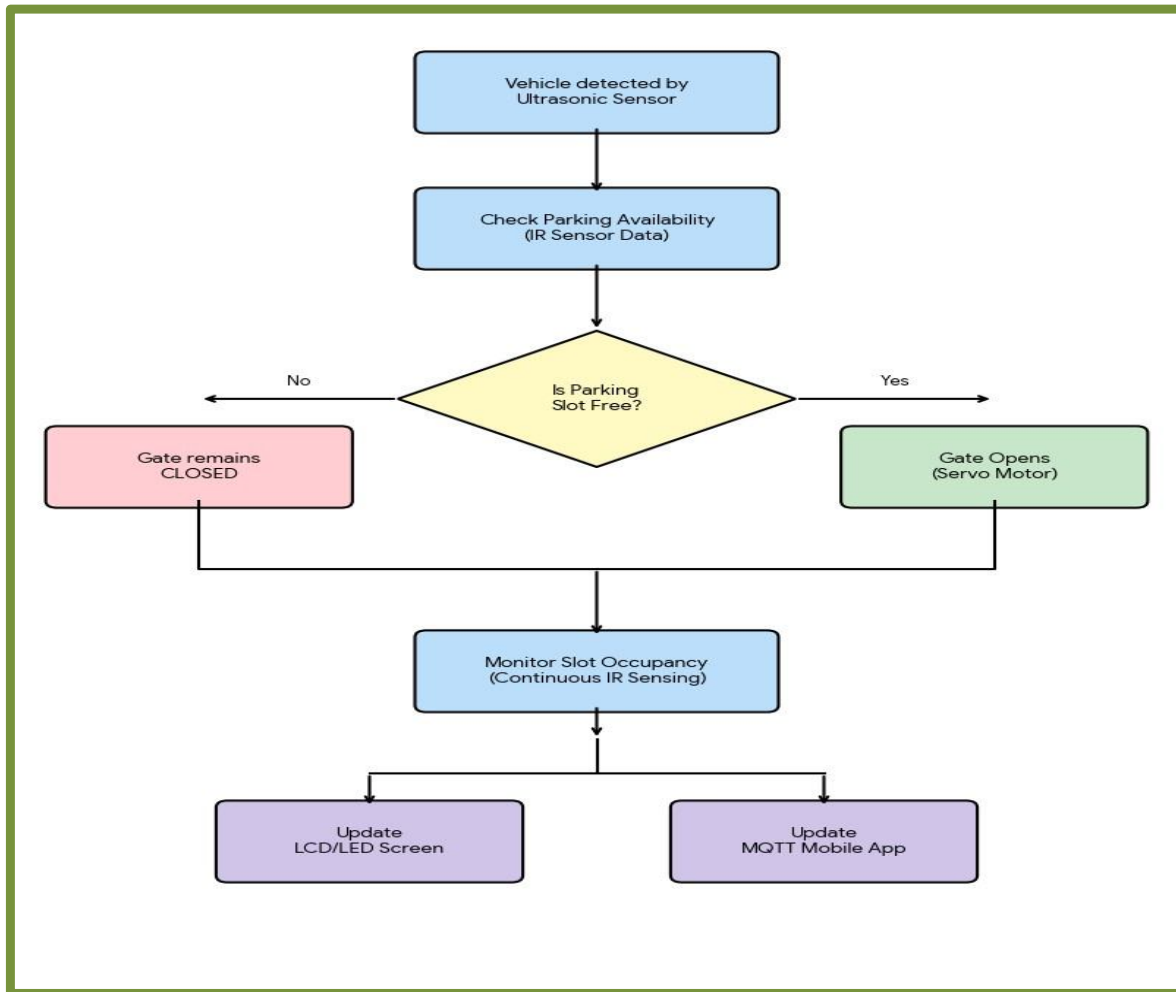
Fig. 2 Working process flow chart
