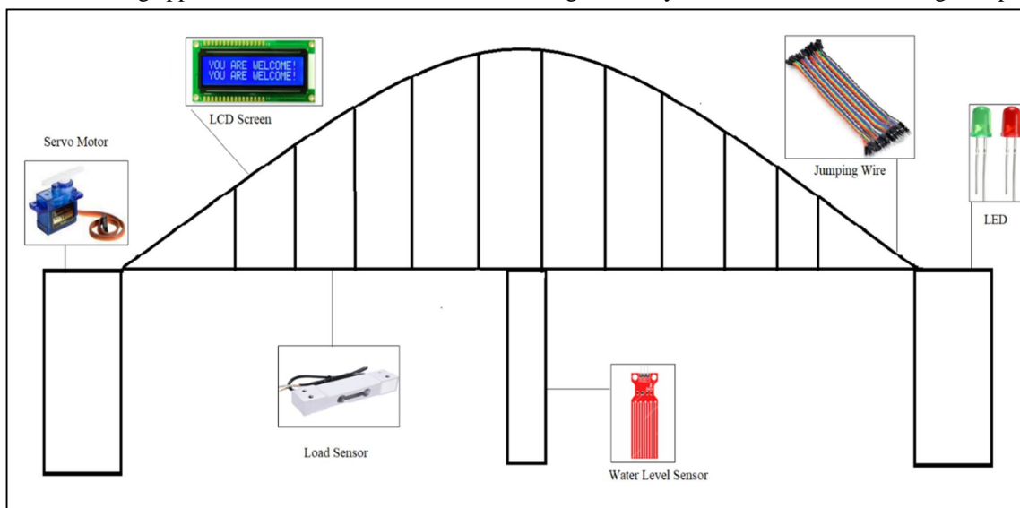
Fig.1 Placement of hardware components on the bridge
