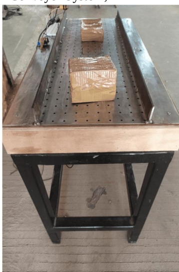
Fig : 5 : Actual Air Conveyor With Conveying Products
