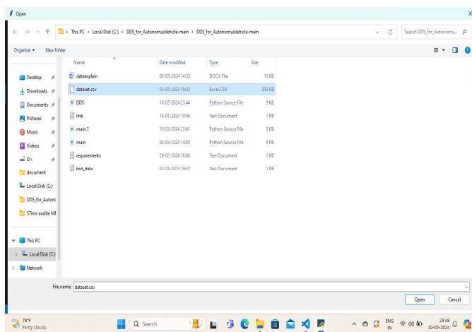
Figure 4: Upload Dataset
