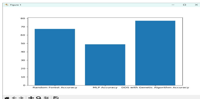
Figure 10: Accuracy Comparison Graph
