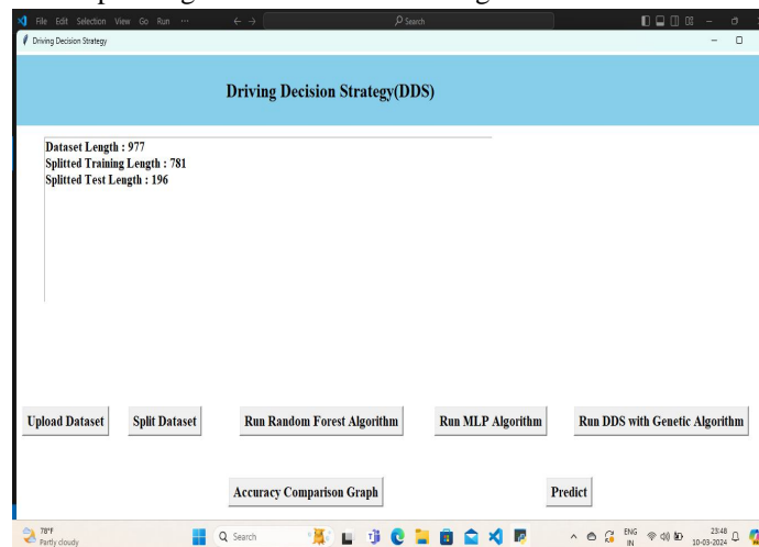
Figure 6: Split Dataset
