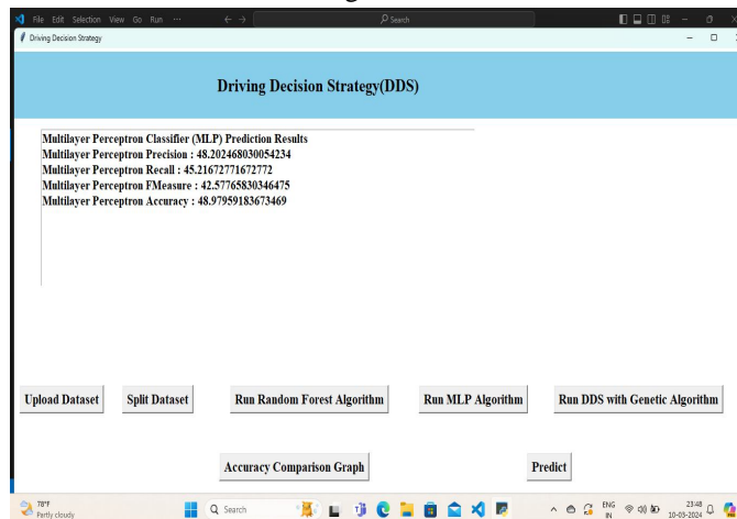
Figure 8: MLP Algorithm
