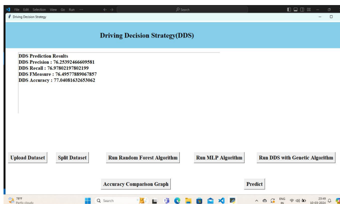
Figure 9: Run DDS with Genetic Algorithm
