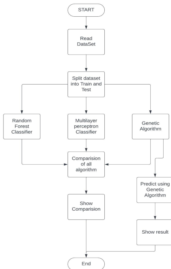
Figure 1: Flow Chart of Determine the Decision Driving Strategy of an Autonomous vehicle
