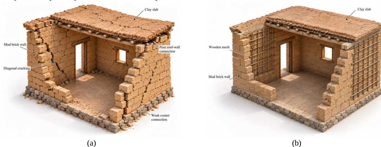
Fig. 1 Three-dimensional models of adobe housing framework: (a) conventional unreinforced adobe building; (b) improved adobe building incorporating wooden mesh reinforcement
