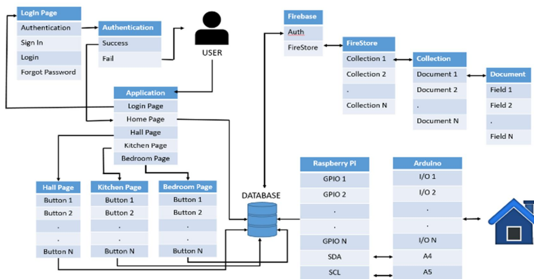
Figure 1: System Architecture
