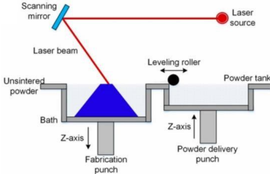
Fig 3. Diagram of SLS from laser sintering to 3D CAD design. Reproduced with permission from Dipta et al., Journal of Manufacturing and Materials Processing , 9(8), 269. (2025). Copyright 2025 Authors, licensed under a Creative Commons Attribution (CC BY) license.
