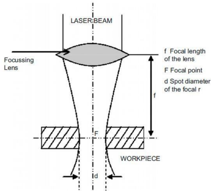
Fig 1. Beam profile schematic for laser beam machining applications. Reproduced with permission from Pramanik et al., Metals , 13(9), 1536. (2023). Copyright 2023 Authors, licensed under a Creative Commons Attribution (CC BY) license.
