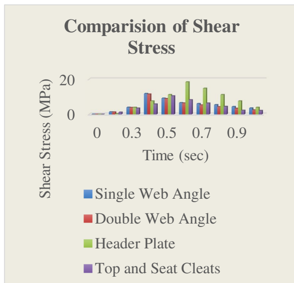
Graph 5: Shear Stress
