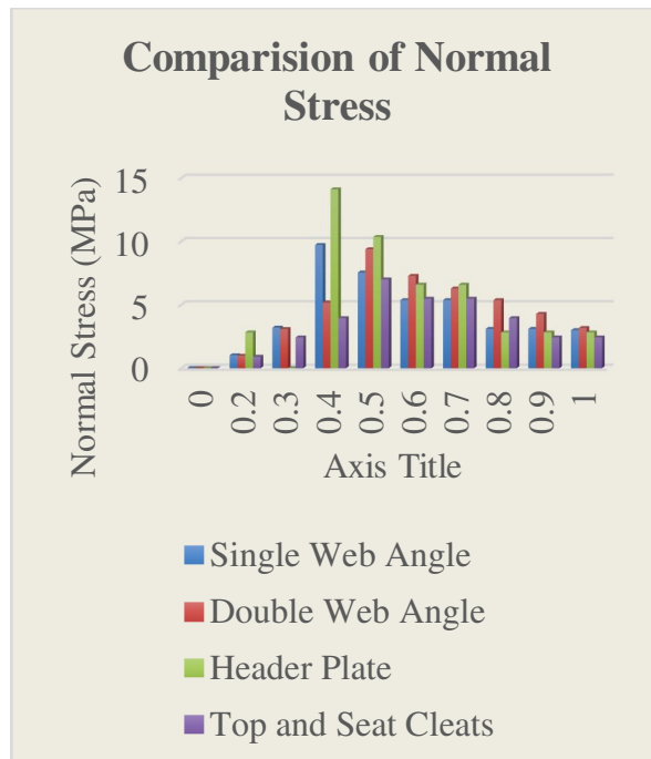
Graph 4: Normal Stress
