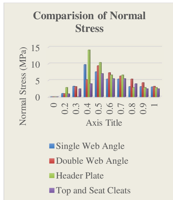
Graph 4: Normal Stress
