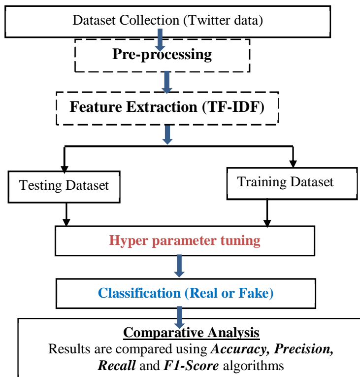
Fig.1. Social Media Text Classification
