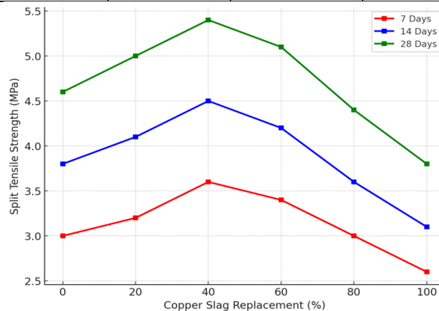
Fig. 5: Split Tensile Strength Test Results
