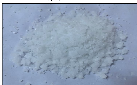
Sodium hydroxide
