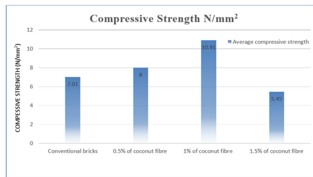
Fig 9 Average Compressive Strength of bricks
