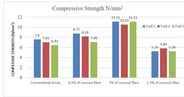
Fig 8 Comparison Between Conventional Brick and Coconut Fibre Bricks
