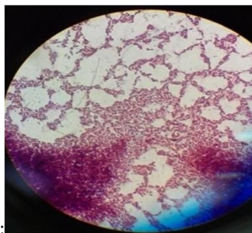
Figure 1: Bacillus Subtilis
