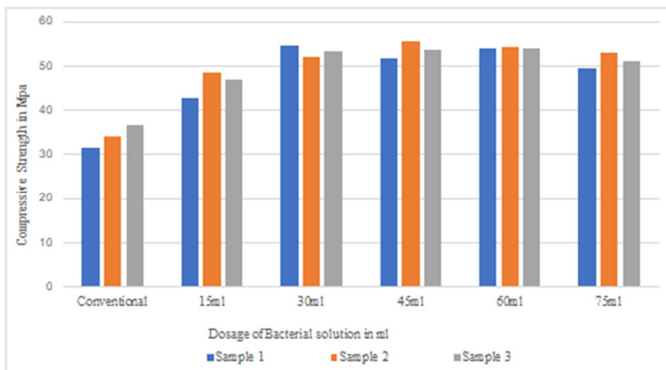
Figure 5: Compressive Strength graph for 28 days
