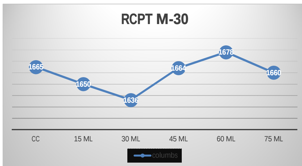
Figure 6: RCPT coulombs
