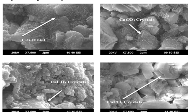
Figure 7: 7 days bacterial concrete effects on SEM
