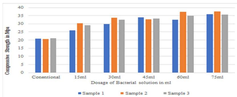
Figure 3: Compressive Strength Graph for 7 Days
