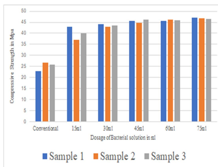
Figure 4: Compressive Strength graph for 14 days
